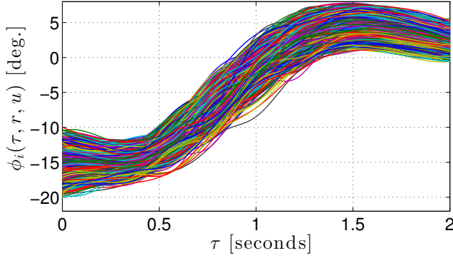
Fig. 2. One hundred roll-angle trajectories over a T_s = 2 second ZOH period resulting from an increase of \Delta = 15^\circ from the previous roll-angle setpoint of u_{k-1} = r_k = -15^\circ . Moreover, the current setpoint is u_k = 0^\circ .
