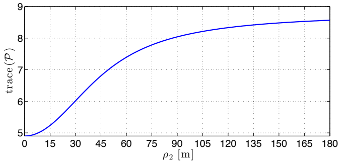
Fig. 8. Cost function g(z) = \text{trace}(\mathcal{P}) with the target located at the origin and the first UAV located on top of the target at an altitude of 40 [m]. Note that the separation angle \gamma is 0 since the first UAV's planar distance is \rho_1 = 0 ; consequently, the fused GEC is completely characterized by the second UAV's planar distance \rho_2 from the target. The second UAV has an altitude of 45 [m].
