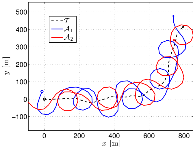
Fig. 11. Uncoordinated trajectories over a three minute window. The starting positions of all vehicles are marked by an “o” while the ending positions are denoted by an “x”. The remaining notation, initial conditions, and target trajectory are the same as in Figure 9.
