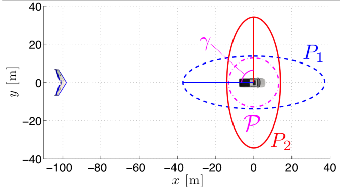
Fig. 5. Individual error ellipses P_1 and P_2 corresponding to the vision measurements from the blue and red UAVs having (x, y, z) coordinates (in meters) of (-100, 0, 40) and (0, 100, 45) respectively, where the latter UAV is not shown. Also depicted by the magenta, dash-dot line is the error ellipse \mathcal{P} corresponding to the combination (fusion) of the measurements obtained from both UAVs, and the separation angle \gamma .
