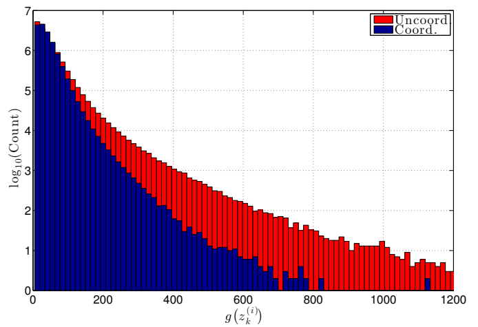
Fig. 15. Histogram of the stage-cost (not averaged over time) for 50,000, 10-minute Monte Carlo simulations. The outlying costs of the uncoordinated policy are not all shown, as they exceed 2,000 [m 2 ].
