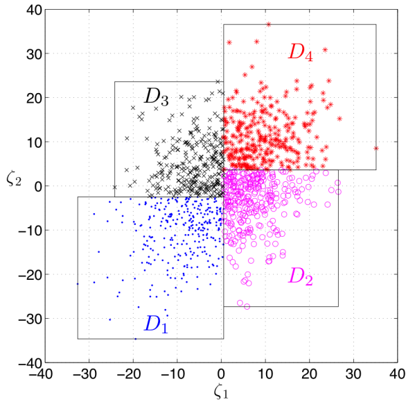
Fig. 7. Partitioning scheme for L = (2, 2) and \zeta^{(i)} \sim \mathcal{N}(0, C) with C \in \mathbb{R}^{2 \times 2} . Here, i \in \{1, 2, \dots, M\} with M = 1, 200 , c_{1,1} = c_{2,2} = 10 , and c_{2,1} = c_{1,2} = 2 . The black rectangles indicate the individual domains. The split in the \zeta_1 coordinate happens roughly at zero to divide the number of points in half, while the splits in the \zeta_2 coordinate further subdivide the points such that each bin contains 300 samples.
