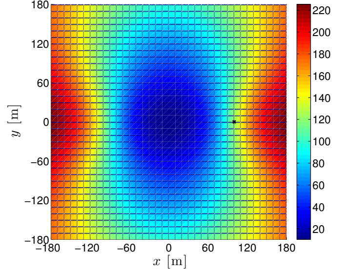
Fig. 6. Cost function g(z) = \text{trace}(\mathcal{P}) with the target located at the origin and the first UAV located at three dimensional position (x, y, z) = (100, 0, 40) , where this UAV's (x, y) position is indicated by a black "x." The second UAV has an altitude of 45 [m], and the (x, y) coordinates in the plot represent its planar position.
