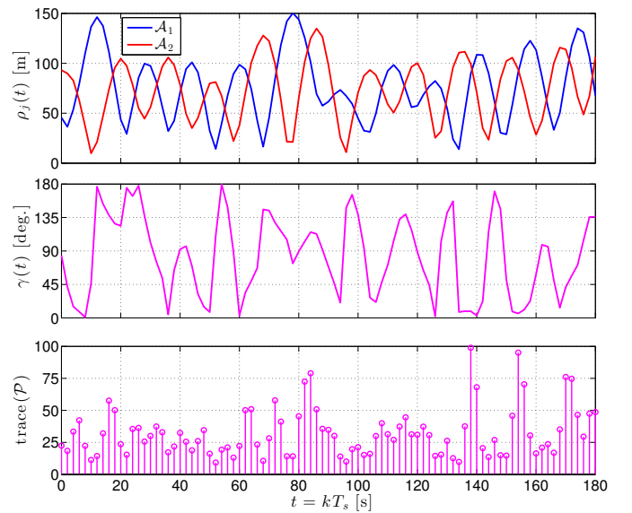
Fig. 10. Performance metrics of optimally coordinated UAVs: planar distances \rho_j , separation angle \gamma , and trace of the fused GEC \mathcal{P} .
