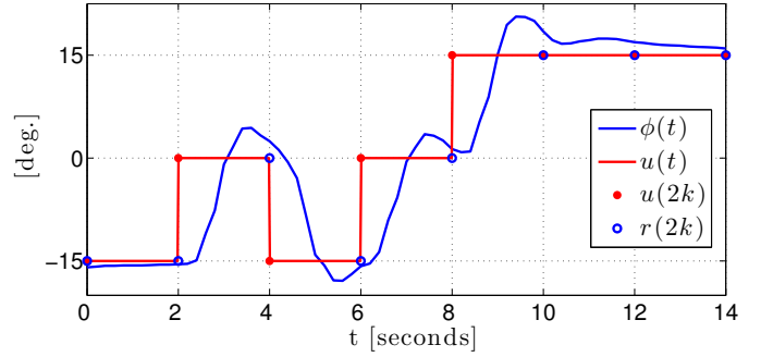
Fig. 1. Monte Carlo simulations to sample roll trajectories. Once every T_s = 2 seconds the roll-angle setpoint is randomly changed to u(kT_s) \in U(r(kT_s)) , where each element of U(r(kT_s)) occurs with equal probability and \Delta = 15^\circ is the maximum allowable change in roll-angle setpoints.
