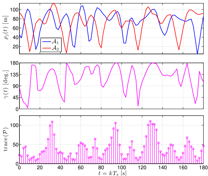
Fig. 12. Performance metrics of uncoordinated UAVs: planar distances \rho_j , separation angle \gamma , and trace of the fused GEC \mathcal{P} .
