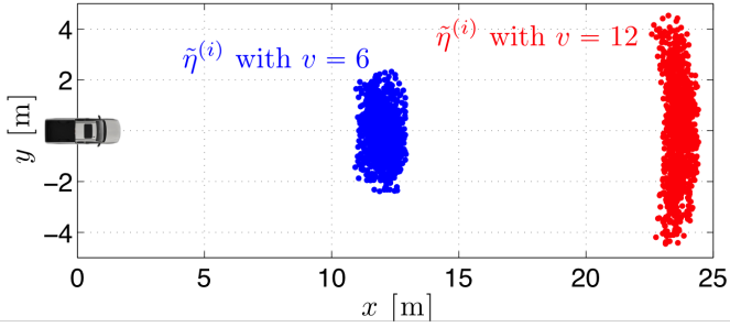
Fig. 4. Sample positions generated from the stochastic target motion model. The two initial target states depicted with different colors correspond to identical initial positions at the origin, but two distinct initial speeds of 6 and 12 [m/s]. For each initial condition, 1,000 samples are generated.
