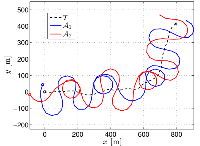
Fig. 9. Optimally coordinated trajectories over a three minute window. The starting positions of all vehicles are marked by an ‘‘o’’ while the ending positions are denoted by an ‘‘x’’. The target (denoted by \mathcal{T} ) begins at the origin travelling at approximately 5.4 [m/s] and finishes its trajectory travelling at approximately 7.3 [m/s]. Both UAVs (denoted by \mathcal{A}_1 and \mathcal{A}_2 ) begin with zero roll.
