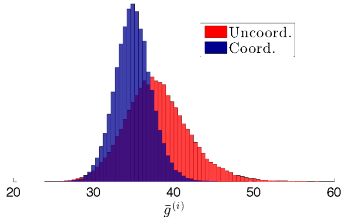
Fig. 14. Histogram of the stage-cost mean \bar{g}^{(i)} = (1/301) \sum_{k=60}^{360} g(z_k^{(i)}) for 10-minutes of steady-state behavior with 50,000 Monte Carlo simulations. The outliers for the uncoordinated policy are not all shown, as they extend out to nearly 73 [m 2 ].
